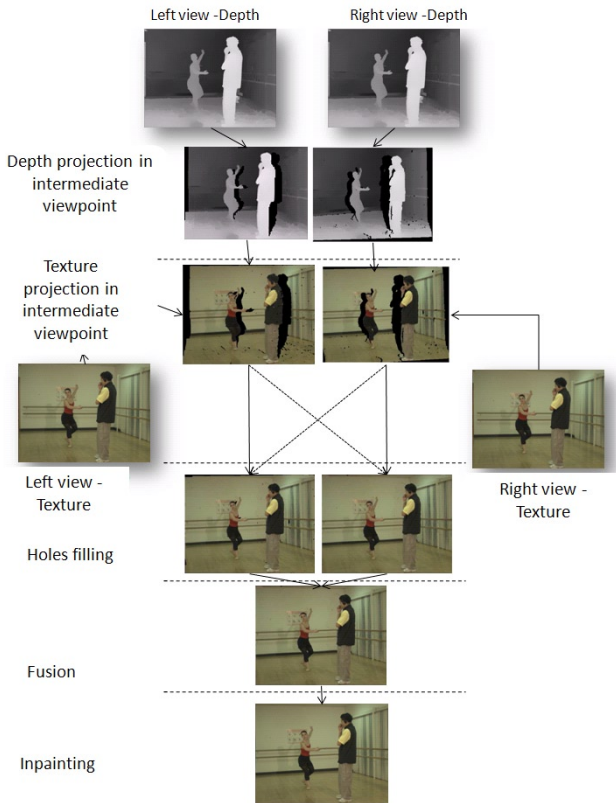
Fig. 2. View synthesis with VSRS.
