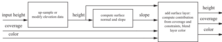
Figure 1: Applying a surface layer includes modification of the elevation data, normal/slope computations, and finally the determination of the new surface color and height value.
