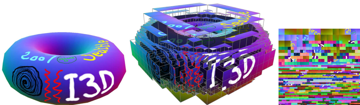
Figure 1: Left : A torus is textured by a TileTree. Middle : The TileTree positions square texture tiles around the surface using an octree. At rendering time, the surface is projected onto the tiles. Right : The tile map holding the set of square tiles.
