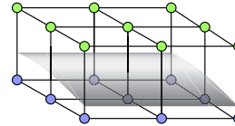
Figure 3: Correct tri-linear interpolation in a volume requires storing the surface as a thick layer. However, the bottom (blue) samples should be sufficient to texture the surface, leading to a 2x saving.
