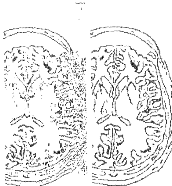
Figure 4: 3D edge detection is more robust and coherent than 2D edge detection: left, we show the result of 2D edge detection performed in successive cross-sections which were orthogonal to the plane of the picture. Result from one cross-section to the next is not as coherent as it is with 3D edge filtering (right) where none of the 3 principal directions is privileged. (Courtesy of G. Malandain and O. Monga)
