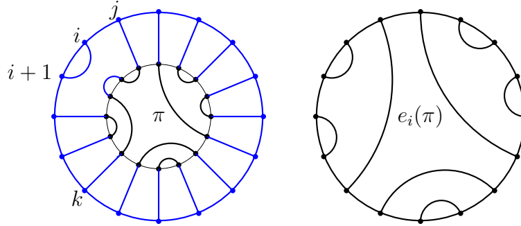
FIGURE 2. Temperley-Lieb action
