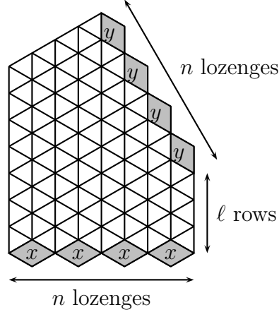
FIGURE 10. Interpretation of \mathcal{R}_\ell(n; x, y)
