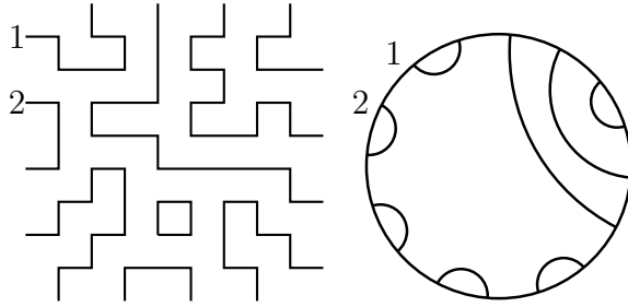
FIGURE 1. An FPL of size 8 and its coupling
