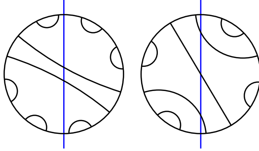
FIGURE 3. Half-turn symmetric couplings of odd (left) and even (right) size
