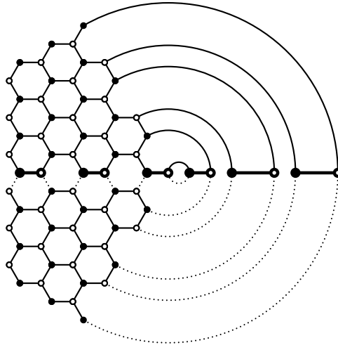
FIGURE 5. Honeycomb lattice version of the graph in Figure 4
