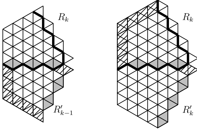
FIGURE 9. Decomposition by symmetry of G_6 and G_7 .
