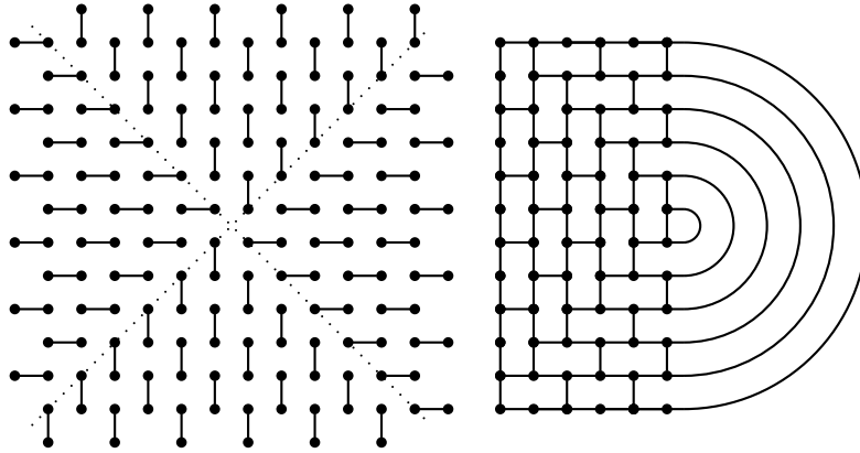
FIGURE 4. Fixed and non-fixed edges in even size
