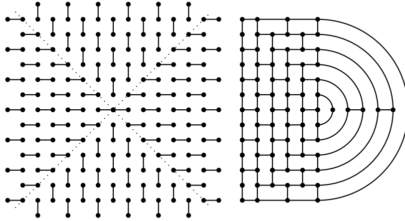
FIGURE 6. Fixed and non-fixed edges in odd size
