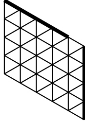
FIGURE 8. The region G_4 .
