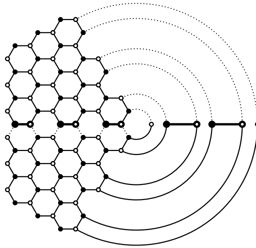
FIGURE 7. Honeycomb version of the graph in Figure 6
