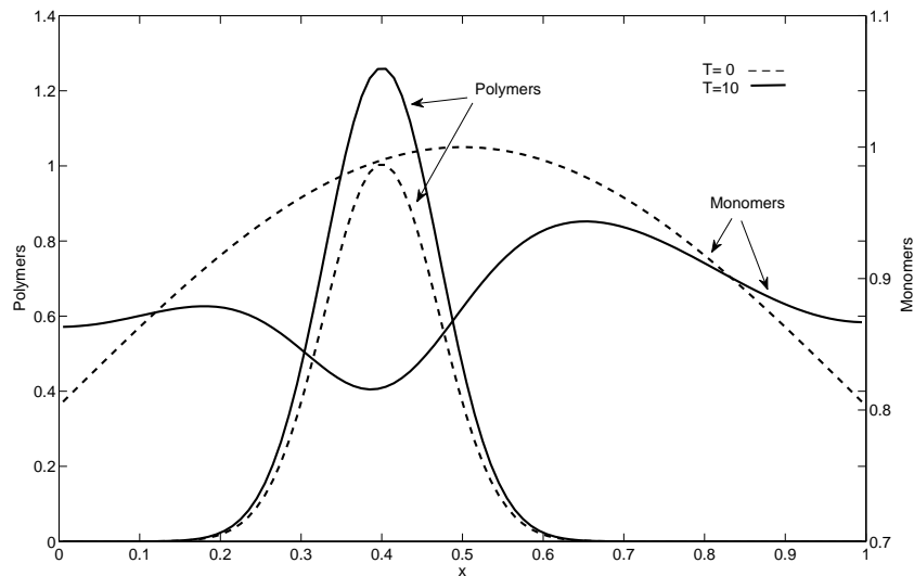
Figure 2: Mass of polymers and density of monomers according to x .
