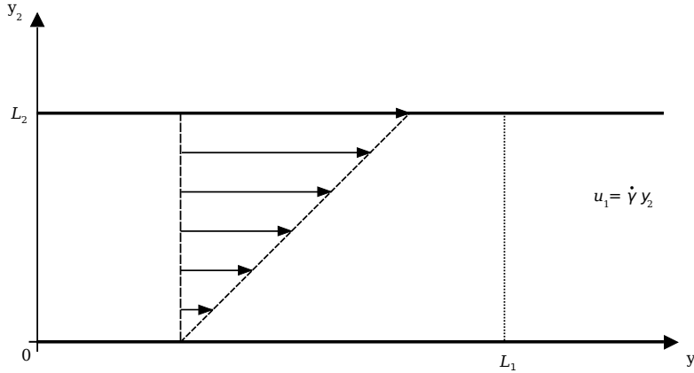
Figure 1: Shear flow: intersection with plane y_3 = c \in (0, L_3) .
