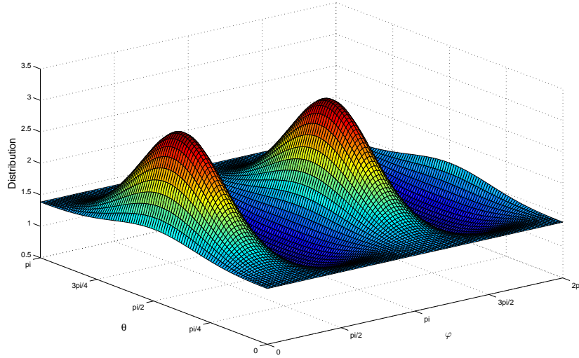
Figure 4: Probability configuration of polymers at x = 0.4 and r = 0.4 for \theta \in (0, \pi) and \varphi \in (0, 2\pi) .
