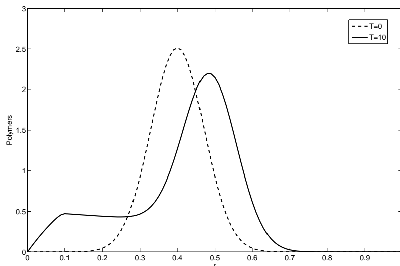
Figure 3: Size distribution of polymer, integrate over the sphere and the space.
