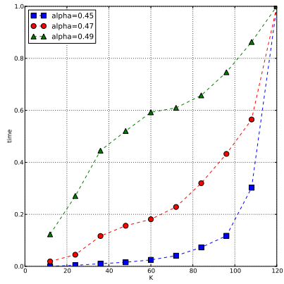
(a) K vs Execution Time Normalized
