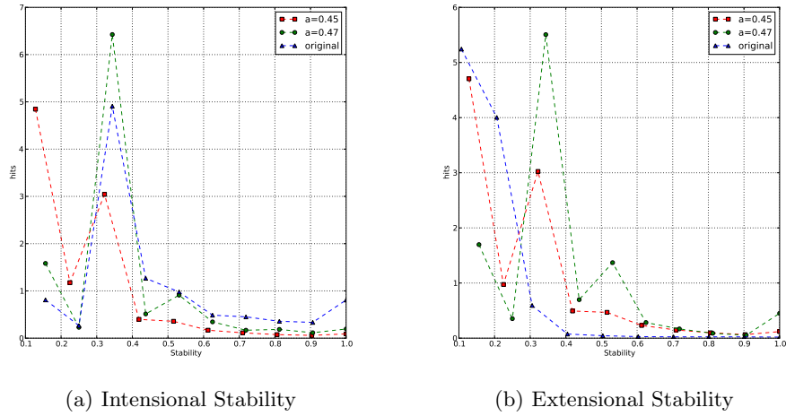
Fig. 4. Stability distribution (k=60)
