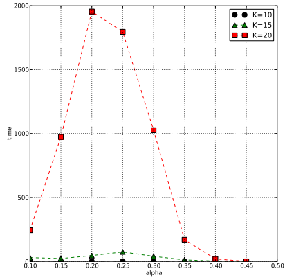
(a) alpha vs Execution Time
