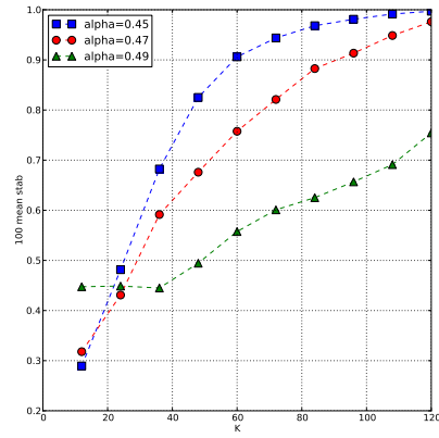
(b) K vs Top 100 Mean Stability
