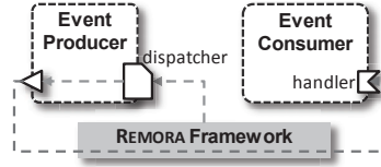
Fig. 8. Event processing scheme in REMORA.
