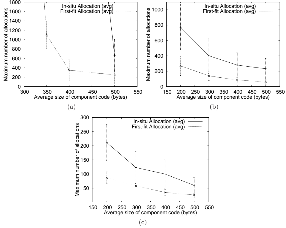
Fig. 21. Memory allocation increase vs. average component size given that the size of deployed software is: a) 38 KB, b) 40 KB, and c) 42 KB.
