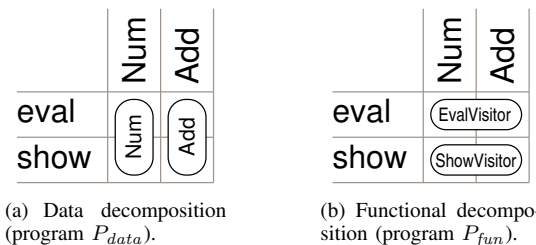
Fig. 3. Coverage of classes with respect to operations and data type.
