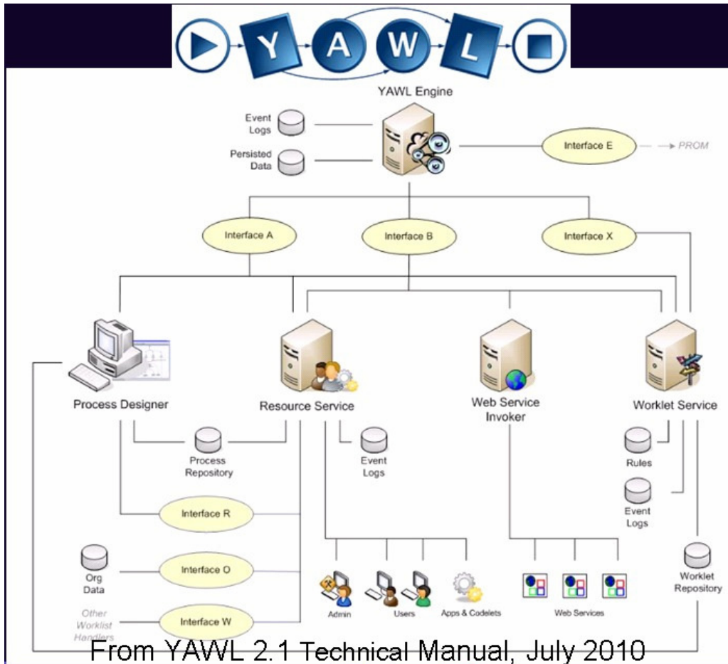
Figure 6. YAWL architecture.
