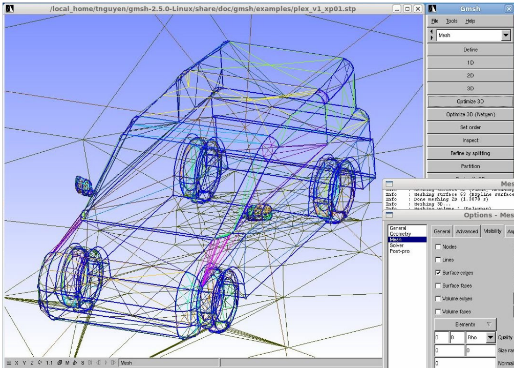
Figure 21. Mesh for vehicle aerodynamics simulation (Gmsh screenshot).
