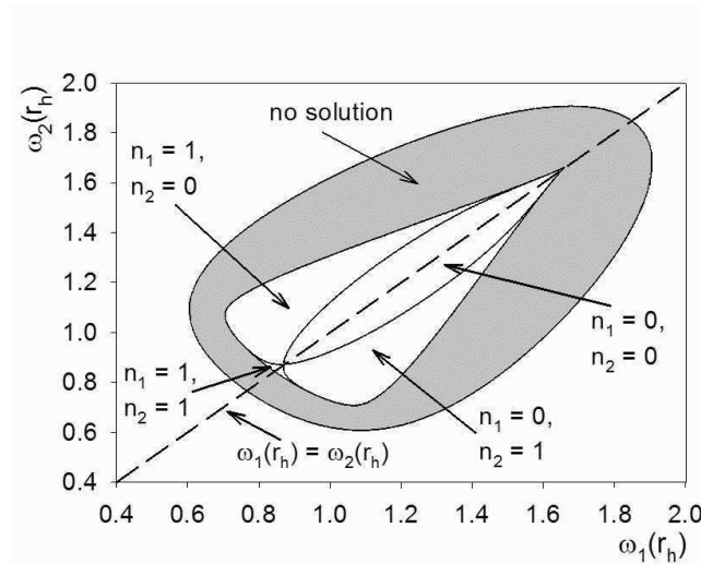
Fig. 9 Solution space for \text{su}(3) black holes with r_h = 1 and \Lambda = -1 . The shaded region indicates where the constraint (71) is satisfied but we do not find black hole solutions. Outside the shaded region the constraint (71) does not hold. Where there are solutions, we have indicated the numbers of zeros of the gauge field functions within the different regions. For this value of \Lambda there is a large region in which both gauge field functions have no zeros. Taken from [9].
