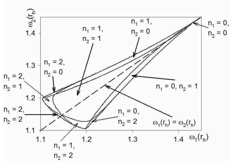
Fig. 8 Solution space for \text{su}(3) black holes with r_h = 1 and \Lambda = -0.1 . The numbers of zeros of the gauge field functions for the various regions of the solution space are shown. For other values of \omega_1(r_h) , \omega_2(r_h) we find no solutions. There is a very small region containing solutions in which both gauge field functions have no zeros, in the top-right-hand corner of the plot. Taken from [9].
