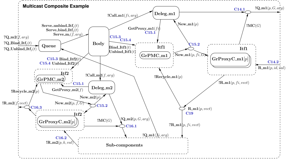
Figure 19: pNets for the Composite component with multicast internal and external interfaces
