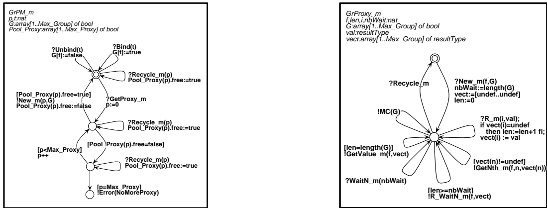
Figure 14: A Group Manager and a Group Proxy
