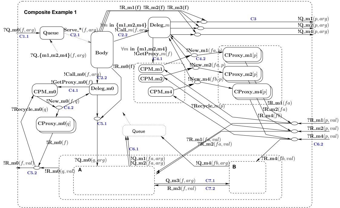
Figure 7: pNet for the Composite Component from Figure 1
