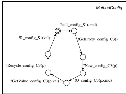
Figure 25: pLTS for the config method of the Local Manager
