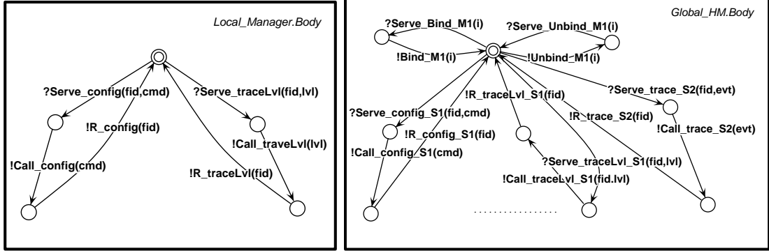
Figure 24: Bodies of the Local Manager (full) and GlobalHM (partial) components
