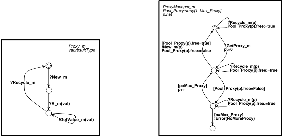
Figure 6: pLTSs for the Future Proxies and Proxy Managers
