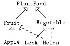
Figure 13: Result of the merging after choosing (d).
