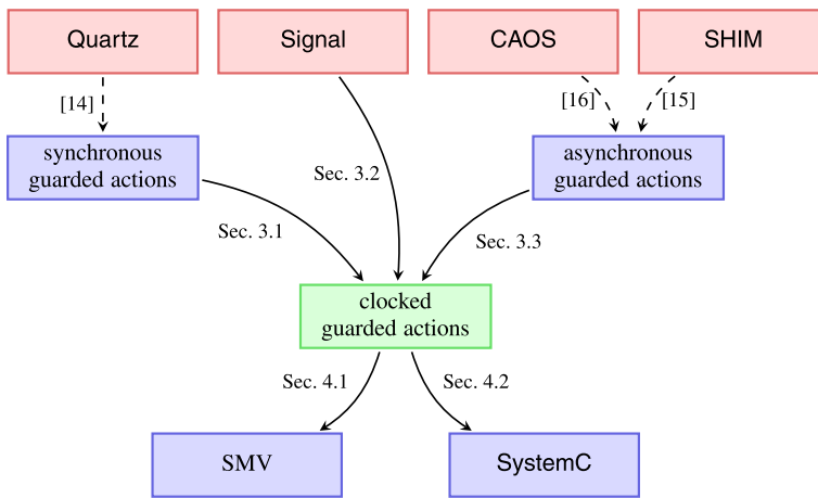
Fig. 1 Design flow for clocked guarded actions
