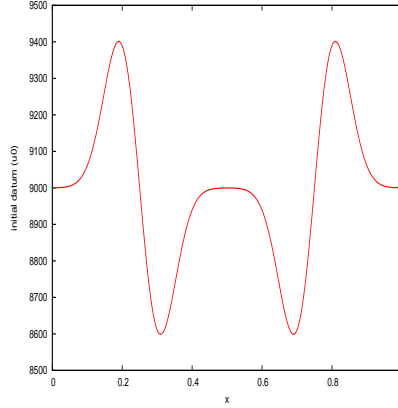
FIGURE 12. The initial condition u_0(x) is a symmetric perturbation of a constant state C_0 = 9000 , the total mass is \mu_0 = 9000 .
