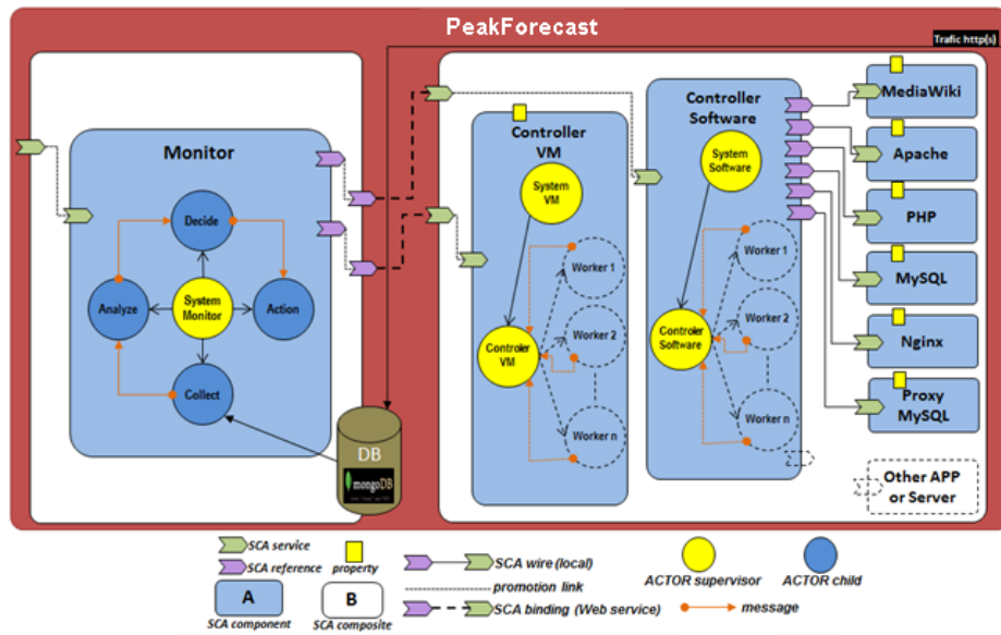
Figure 8: PeakForecast architecture
