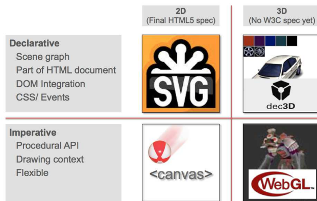
Figure 1: The position of the Declarative 3D approach in the current Web graphics technology ecosystem.
