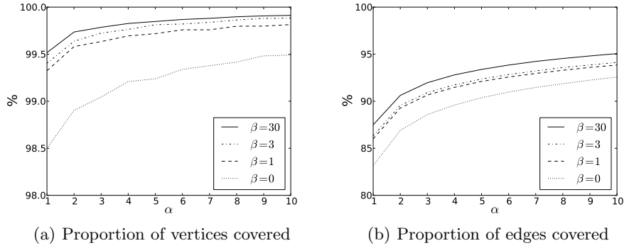
Fig. 3. Proportion of vertices and edges covered when using NTC heuristics.
