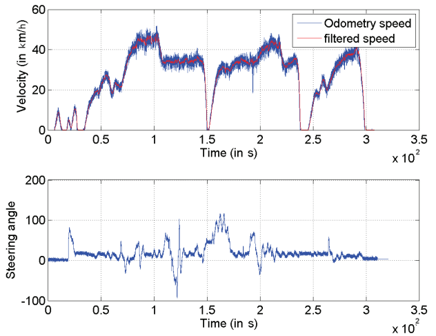
Fig. 8. Vehicle velocity
