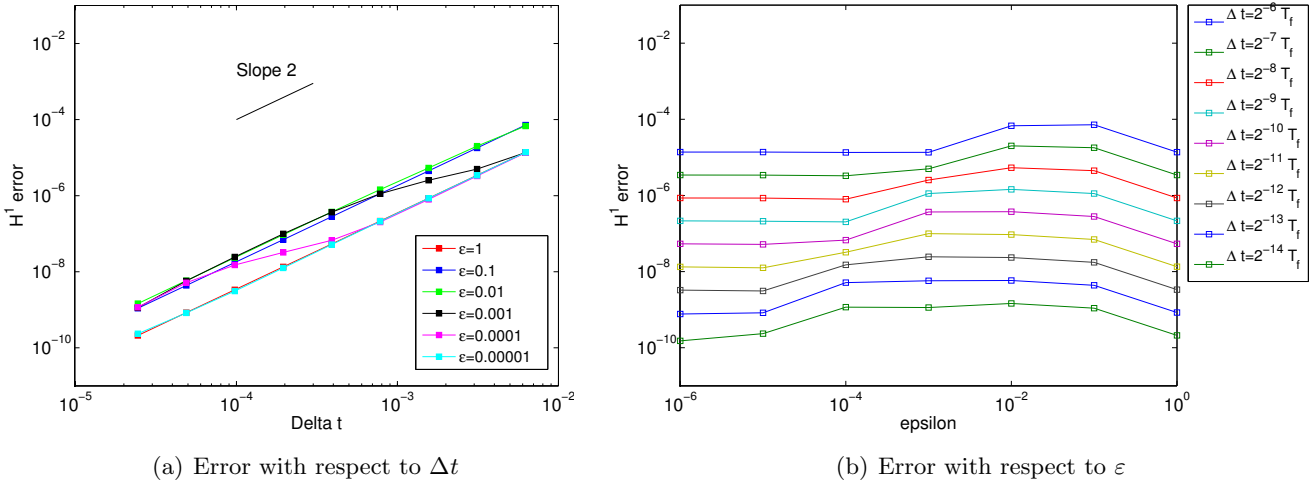
Figure 6: (NKG) H^1 relative error (in log-log scale) for the second order UA scheme with the third order initial data.
