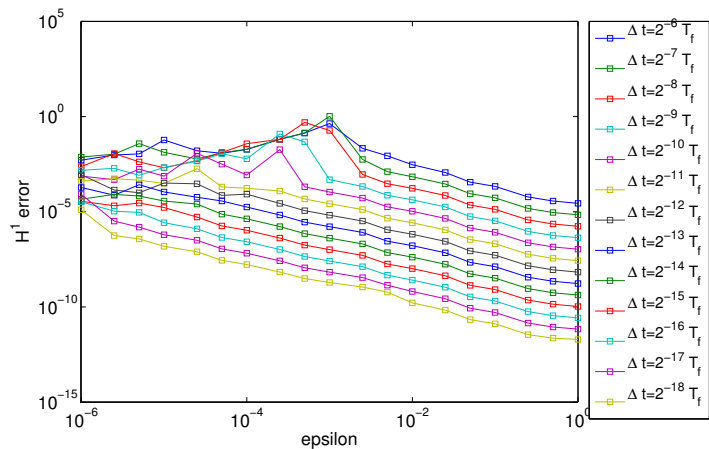
(b) Error with respect to \varepsilon
