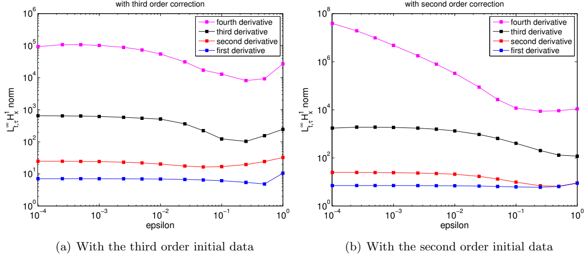
Figure 4: (NKG) L_t^\infty L_\tau^\infty H_x^1 norm (in log-log scale) of \partial_t^k U^\varepsilon(t, \tau, x) with respect to \varepsilon , for k \in \{1, 2, 3, 4\} .
