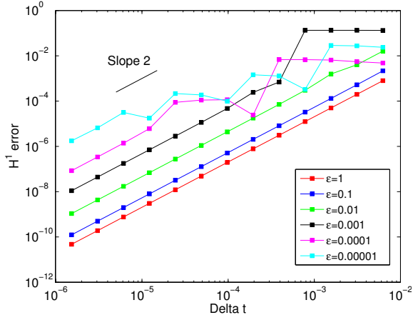
(a) Error with respect to \Delta t
