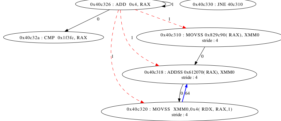
Fig. 3. Code and dependence graph for the loop in function s424 of TSVC benchmark. array is aliased with xx with an offset of 63 floats.
