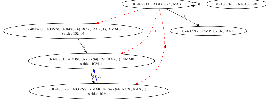
Fig. 2. Code and dependence graph for one loop of function s2233 in TSVC benchmark.
