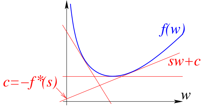
Figure A.1: Convex function f(w) as the maximum of affine functions. For any slope s , c = -f^*(s) is the intercept of the tangent of direction s .
