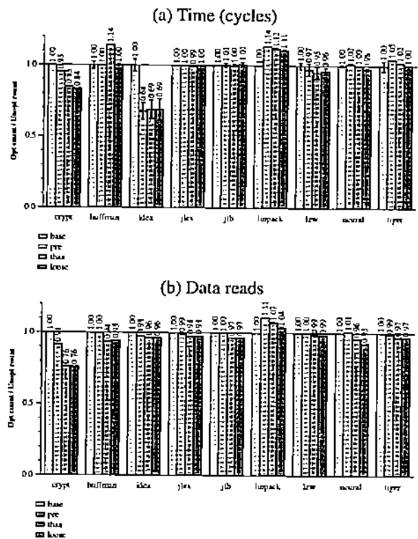
Figure 6: JIT metrics
