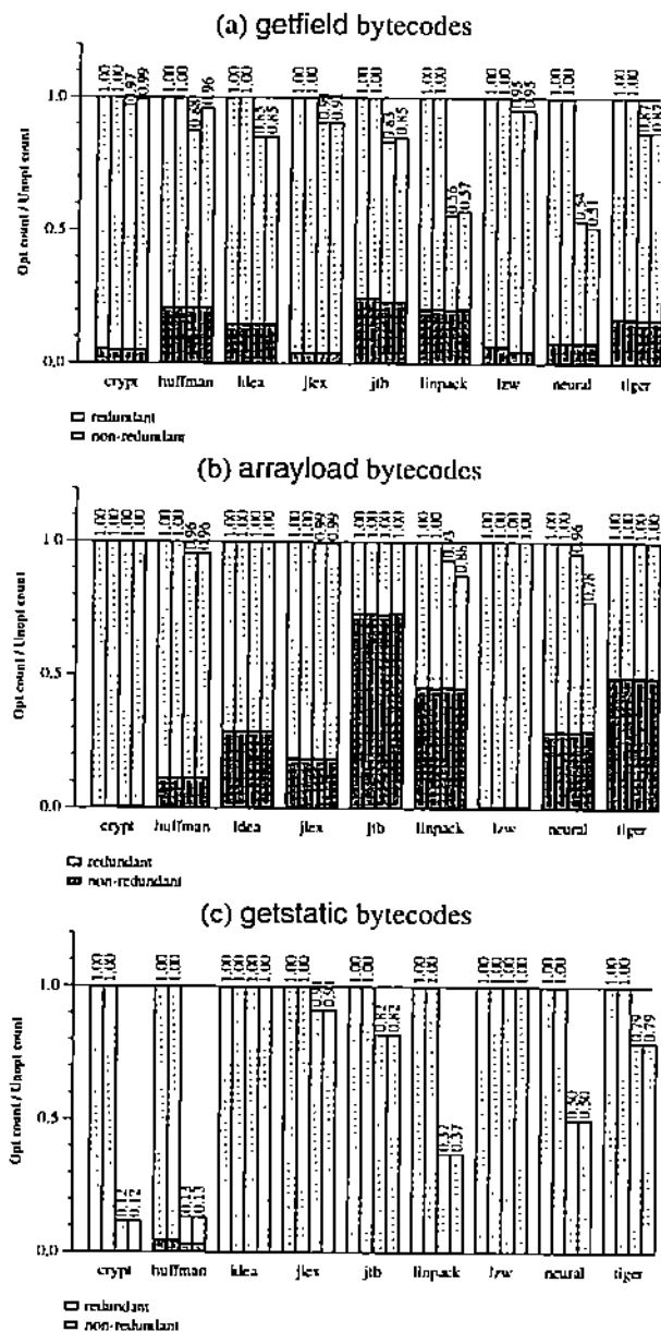
Figure 5: Access bytecodes executed
