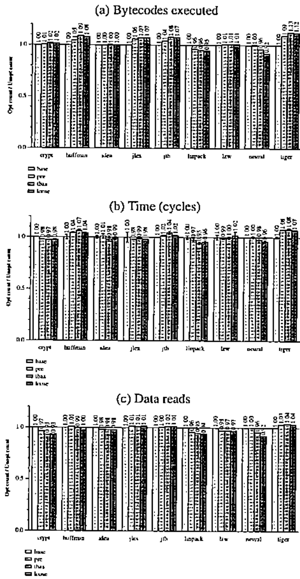
Figure 3: JDK metrics
