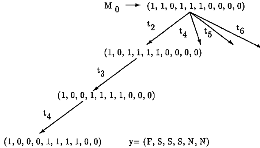
Figure 4: A reachable acceptable state
