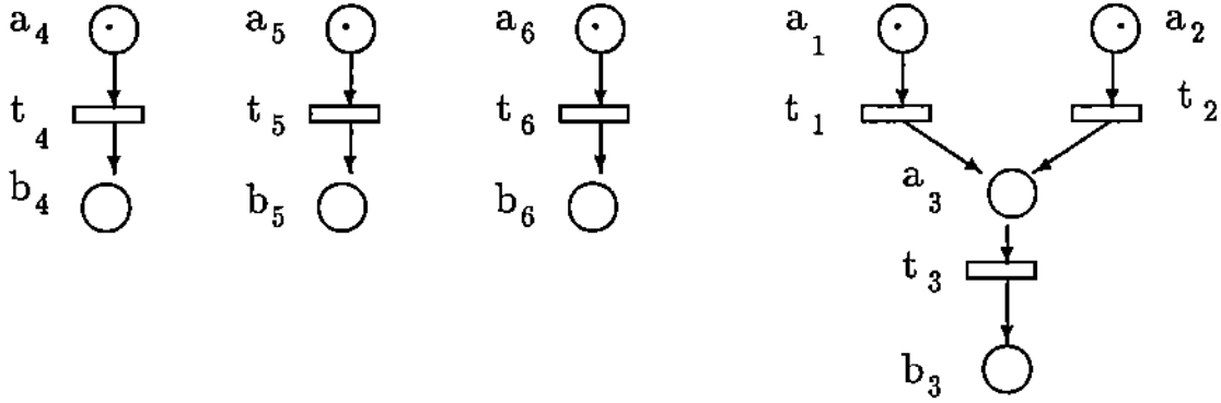
Figure 2: PTN for the travel agent transaction
