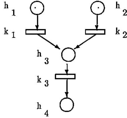
Figure 1: A Predicate Transition Net
