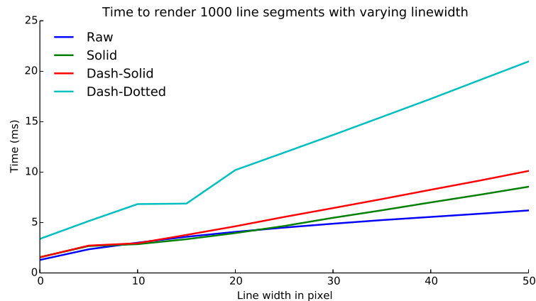
Figure 12. The time to render line segments with increasing line widths is linearly correlated with the line width.
