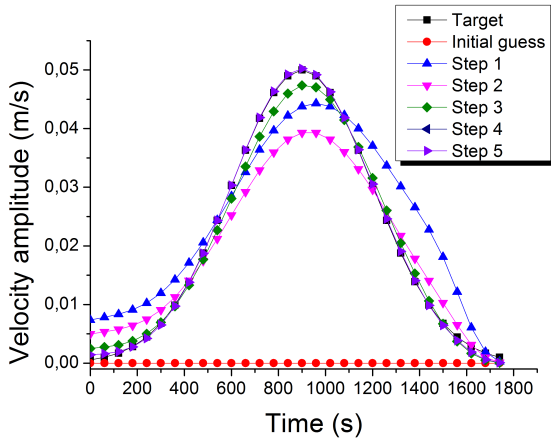
FIGURE 8 – Reconstructed velocity profiles through iterations in the i -loop, for sensor set 1
