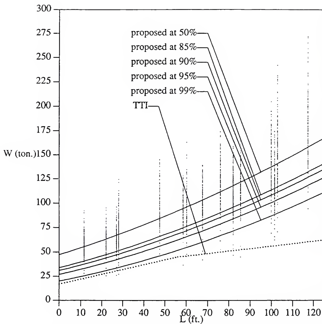
Figure 4.60 Allowable load, W, vs. wheel base, L, for 10 \leq L \leq 120 ft. superimposed on the proposed confidence limits at operating stress level (i.e 36% overstress beyond design stress level) and that by Noel and James (1989) at only 5% overstress for HS20 designed bridges and 30% overstress for H15 designed bridges beyond design stress level
