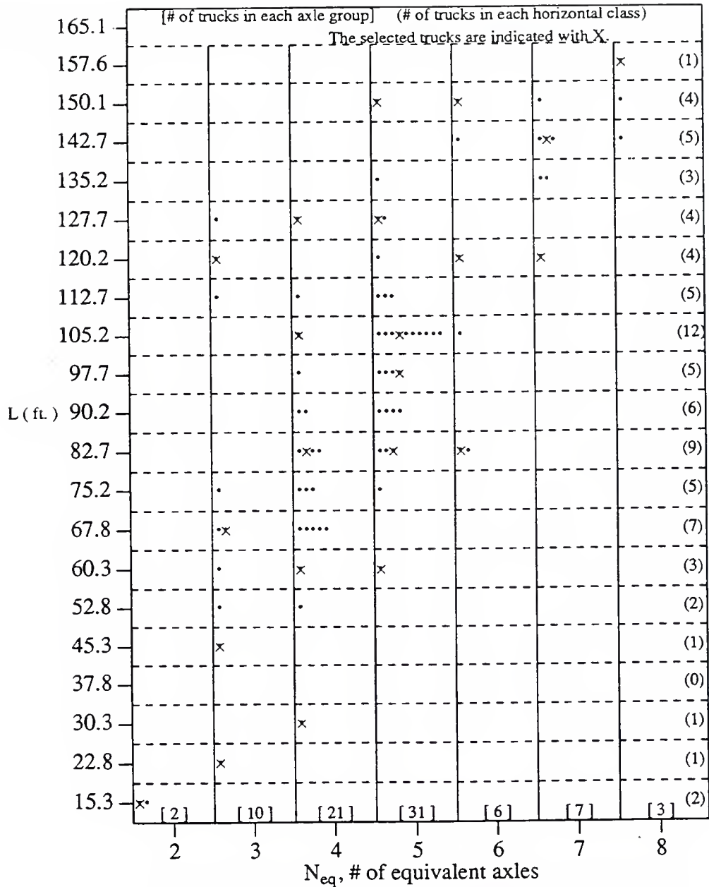
Figure 2.1 Truck population distribution with respect to number of equivalent axles, N_{eq} and wheel base, L.
