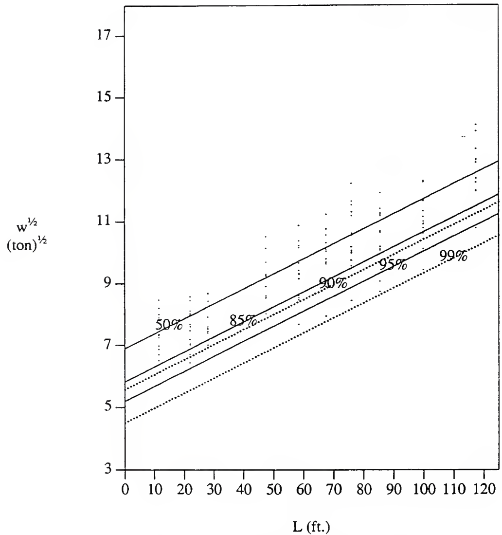
Figure 4.5 Transformed data, w^{1/2} , vs. Wheel Base, L , for test sample of bridges and the predicted w^{1/2} at confidence levels 50%, 85%, 90%, 95%, and 99%
