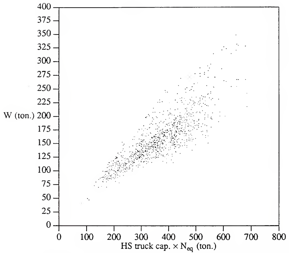
Figure 3.25 Allowable load, W , vs. the product of HS truck capacity and number of equivalent axles, N_{\text{eq}} for 120 < L \leq 160 ft.
