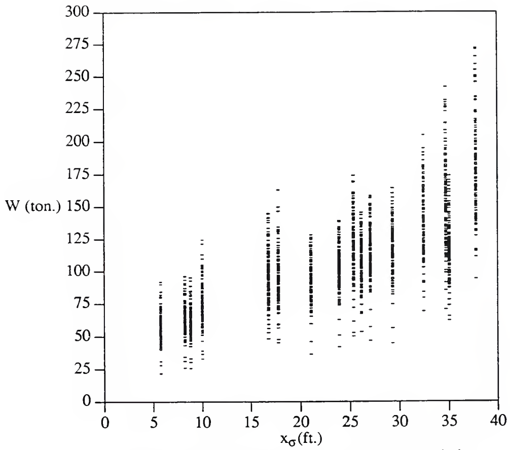
Figure 3.10 Allowable load, W , vs. standard deviation of truck load distribution, x_\sigma , for 10 \leq L \leq 120 ft.
