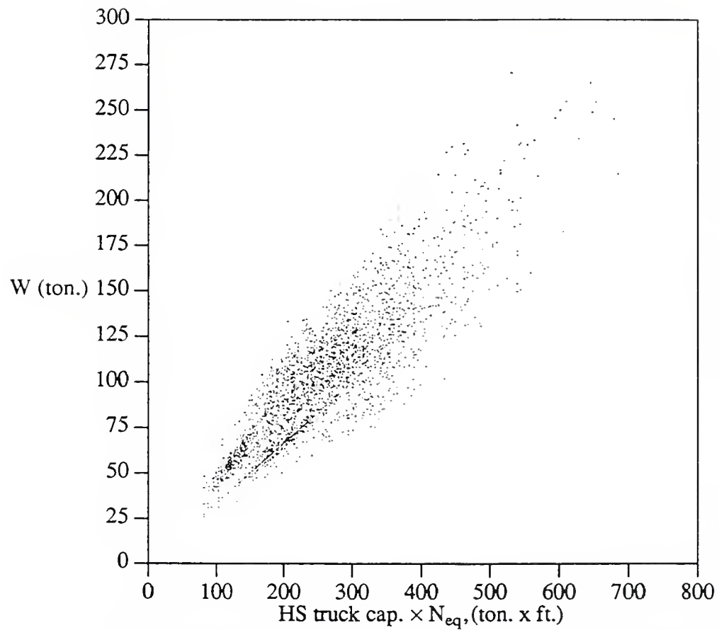
Figure 3.22 Allowable load, W , vs. the product of HS truck capacity and number of equivalent axles, N_{\text{eq}} , for 10 \leq L \leq 120 ft.
