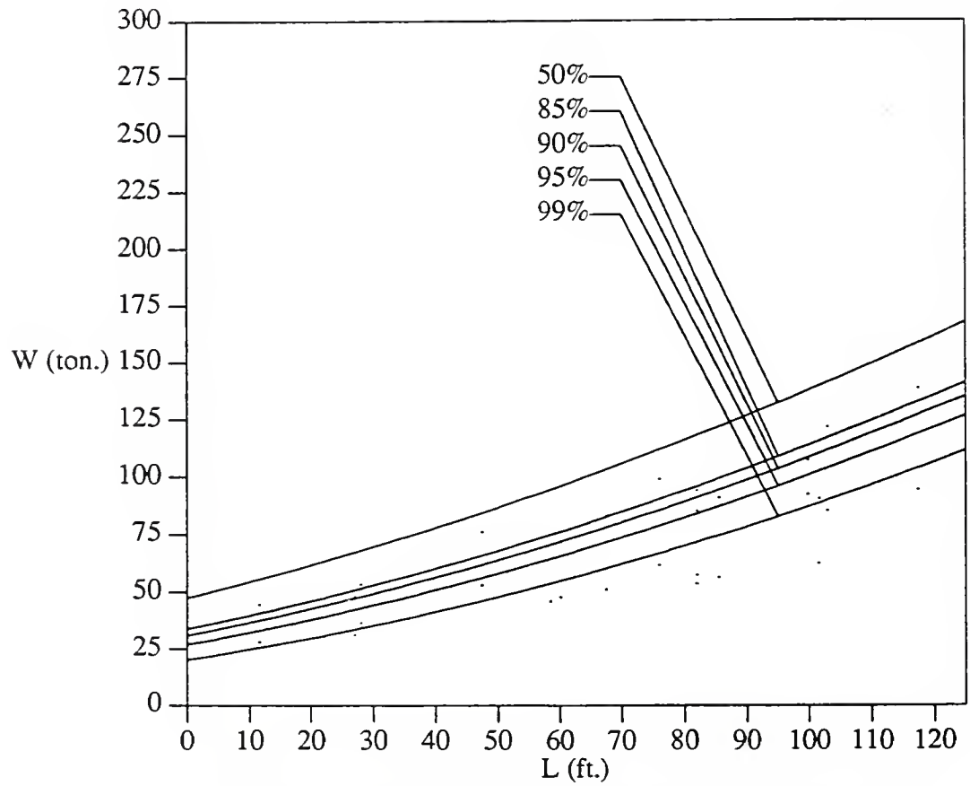
Figure 4.27 Allowable load, W , vs. the wheel base, L , for stt bridges and the confidence limits for all the bridges
