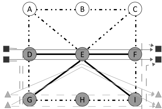
(f) Shared prot smart: 3 nodes and 10 links put to sleep
