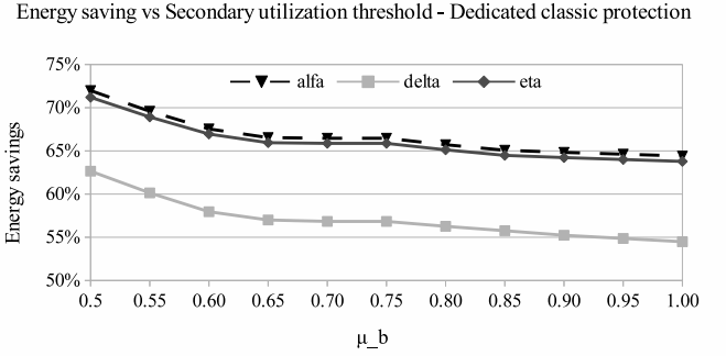
Figure 4: Analysis of the trade-off between energy savings and network congestion, obtained by adjusting the secondary utilization threshold \mu_b from 0.5 to 1 when solving STPH.
