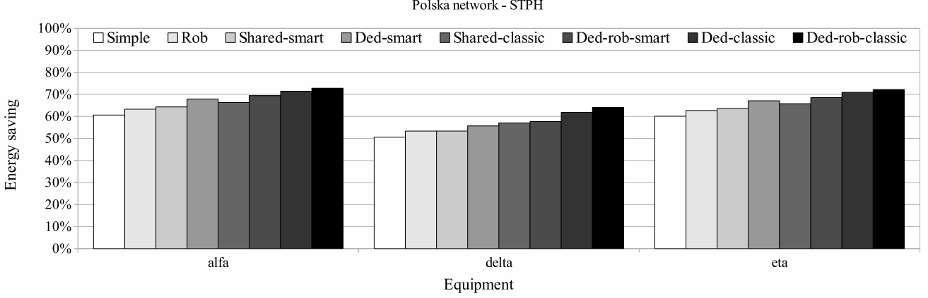
Figure 5: Energy savings achieved by STPH when implementing the different protection schemes on polska instances.
