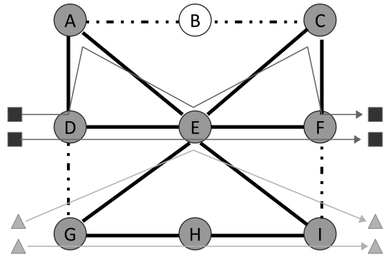
(b) Robust: 1 node and 4 links put to sleep
