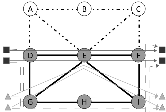
(d) Shared prot: 3 nodes and 6 links put to sleep
