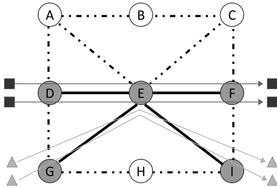
(a) Simple: 4 nodes and 10 links put to sleep
