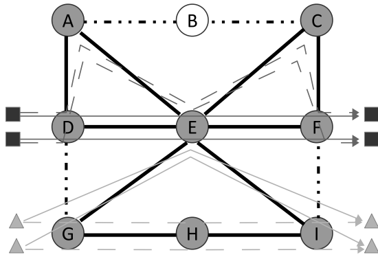
(c) Dedicated prot: 1 node and 4 links put to sleep
