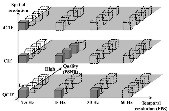
Fig. 1. SVC scalabilities [4].
