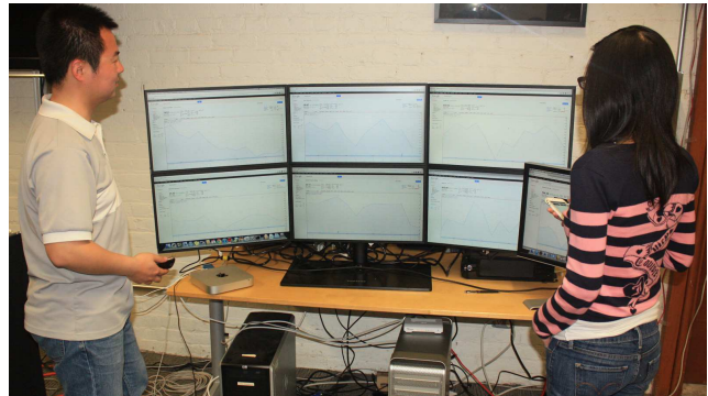
Figure 1: HydraScope enables construction of multi-display meta-applications, controlled by mobile devices.
