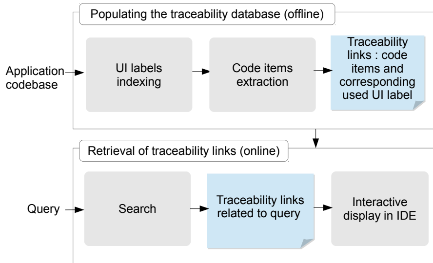
Figure 1: Traceability link extraction overview.
