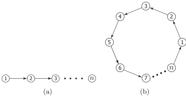
Fig. 6. Two families of directed graphs: (a) Directed path; (b) Directed cycle. Note that the former is weakly connected and not balanced, and the latter is strongly connected and balanced.
