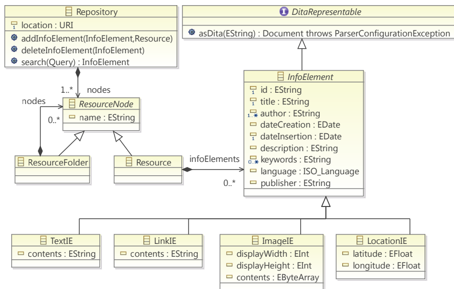
Figure 5: Repository Model
