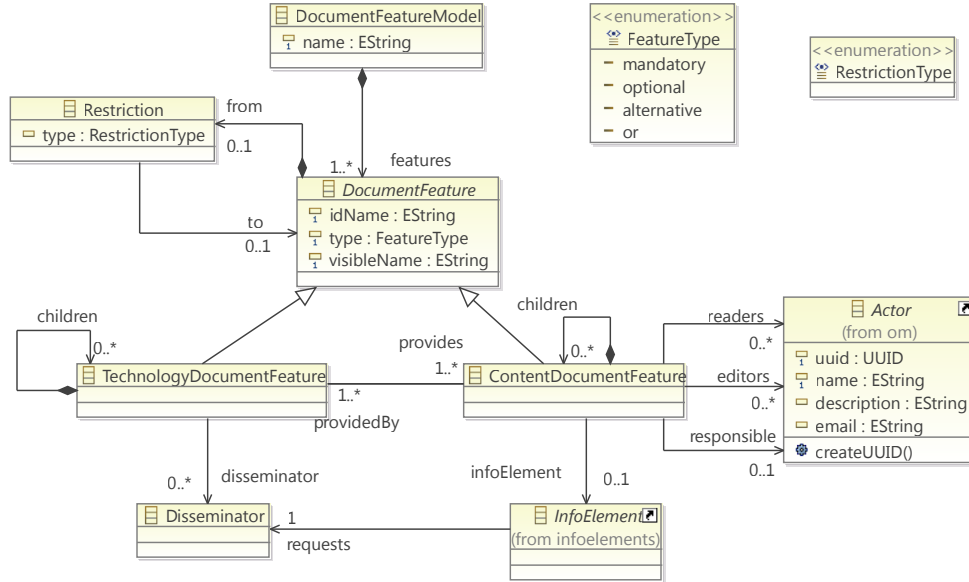
Figure 8: Feature metamodel
