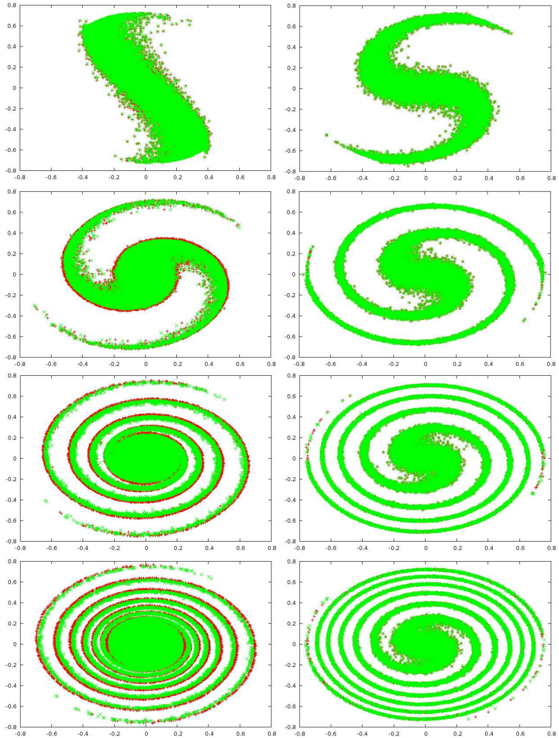
Figure 10: The cases of Vlasov-Poisson ( left ) and of Vlasov with E_\varepsilon = -r^3 ( right ), when \varepsilon = 0.0001 . In red: the reference solution. In green: the solution obtained with the improved ETD scheme. From top to bottom : t = 10 , t = 30 , t = 60 and t = 90 . The time step for the ETD scheme is \Delta t = 0.5 .
