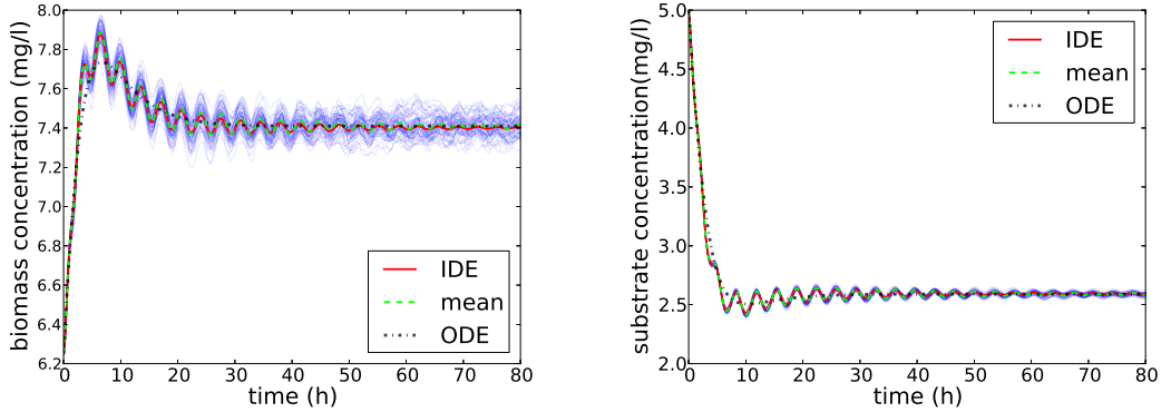
Figure 6: Evolutions of the biomass (left) and the substrate (right) concentrations of 60 independent runs of the IBM (blue), the mean of the IBM (green), the IDE (red), the ODE (black) fitted by the least squares method on the IBM. The parameters of the Monod law (3) of the ODE are \mu_{\max} = 0.537 and K_s = 4.363 . The division rate function is given by the equation (19). \bar{\lambda} = 5 \text{ h}^{-1} , m_{\text{div}} = 0.0005 \text{ mg} , p_\beta = 100 , V = 1.0 \text{ l} , N_0 = 10000 . Other parameters are given in the Table 2.
