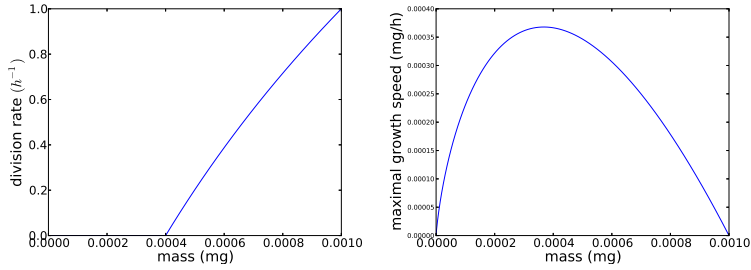
Figure 1: ► (Left) Division rate function \lambda(x) defined by (15) with \bar{\lambda} = 1 \text{ h}^{-1} , m_{\text{div}} = 0.0004 \text{ mg} and p_\lambda = 1000 . ► (Right) Maximal growth speed with the Gompertz growth speed function (14) with r_{\text{max}} = 1.0 \text{ h}^{-1} , m_{\text{max}} = 0.001 \text{ mg} (namely the RHS of the inequality (14)).
