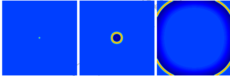
Figure 5. \alpha = -0.1 (upper) : center stimulation, I_{stim}(100, 100) = 1
