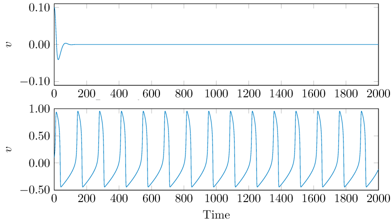
Figure 2. Comparison of \alpha = 0.1 (upper) and \alpha = -0.1 (lower) in FHN model (Eq. (5)). Parameters : \gamma = 0.008 , \varepsilon = 0.01 ; initial conditions : v_{\text{ini}} = 0.1 , w_{\text{ini}} = 0 ; adaptive time step.
