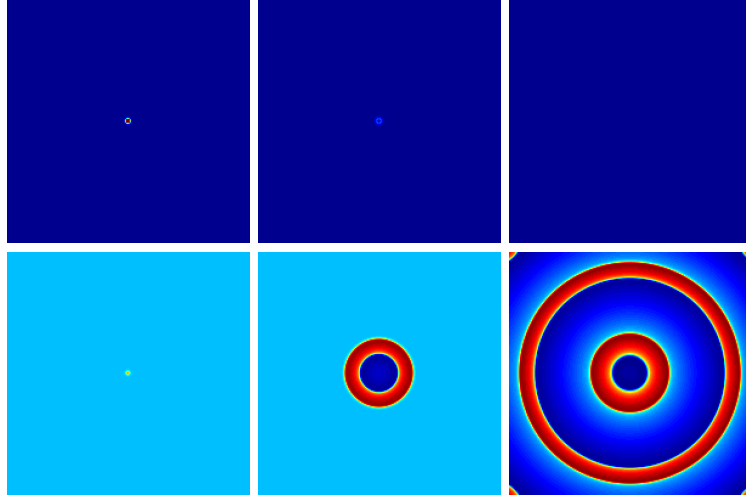
Figure 4. \alpha = 0.1 (upper) and \alpha = -0.1 (lower), center initiation : v_{ini}(100, 100) = 1 , zeros for other cells; w_{ini}(1 : 200, 1 : 200) = 0 .
