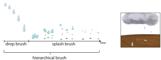
Figure 9: Rain Example. This example shows how complex scenes can be constructed with a hierarchy of simple brushes. A drop and a splash brushes are designed, and combined into a single hierarchical motion brush. On the right, this motion brush is used to fill a scene with rain.
