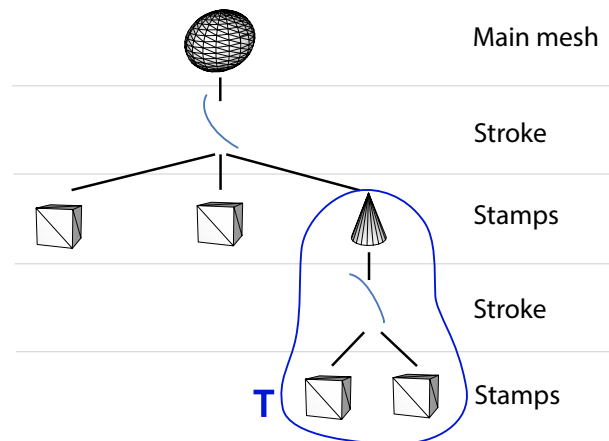
Figure 7: Example of a scene graph using motion brushes. The user created a cube brush and used it to paint a stroke on a cone. The obtained scene was described by the tree T . The painted cone was then used as a motion brush along with the cube brush to paint on a rounder mesh. When instantiating the stamp using the cone brush, T was added as a subtree to the scene hierarchy.
