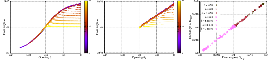
Fig. 3. Left (resp. Middle): scatter plots showing final angle \phi(\varepsilon) and opening \theta_1(\varepsilon) for \rho = -0.7 and S_{\text{norm}} (resp. S_{\text{aug}} ). Every color is for a fixed \delta and variable \varepsilon . Right: Scatter plot showing (\phi(S_{\text{norm}}), \phi(S_{\text{aug}})) .
