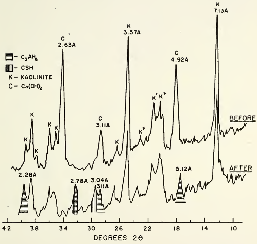
Figure 1-B. X-ray Diffractometer Traces of Ca(OH)_2 -Kaolinite Mixture Before and After Reaction at 60°C.
