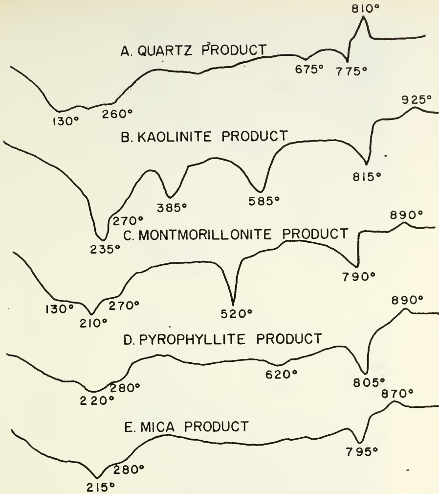
Figure 3. Differential Thermal Analysis of \text{Ca}(\text{OH})_2 -Silicate Reaction Products at 45^\circ\text{C} . Heating Rate Varies from 58^\circ\text{C} to 5^\circ Per Minute.
