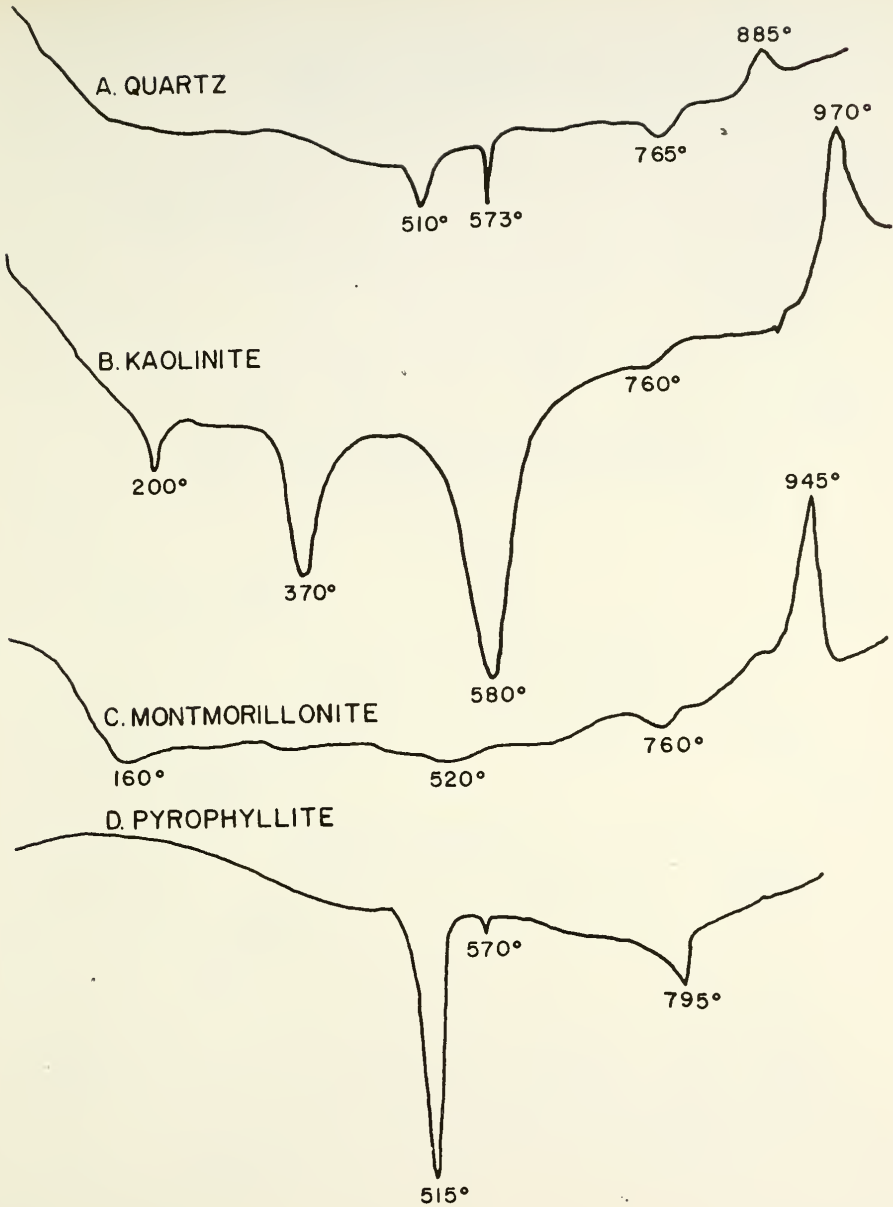
Figure 2. Differential Thermal Analysis of Products of \text{Ca}(\text{OH})_2 -Silicate Reactions at 60^\circ\text{C} . Heating Rate 10^\circ\text{C} Per Minute.
