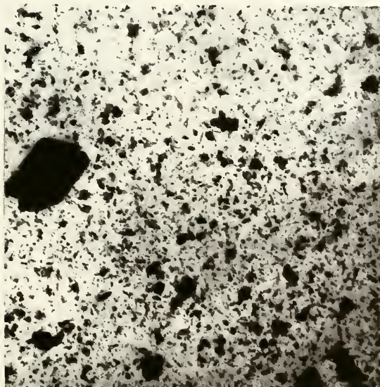
Plate 1. Electron Micrographs of \text{Ca}(\text{OH})_2 -Silicate Reaction Products at 60^\circ\text{C} . (A) Quartz. (B) Kaolinite.
