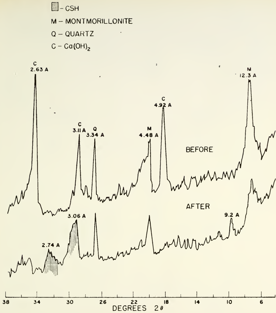
Figure 1-3. X-ray Diffractometer Traces of \text{Ca}(\text{OH})_2 Montmorillonite Mixtures Before and After Reaction at 60^\circ\text{C} .
