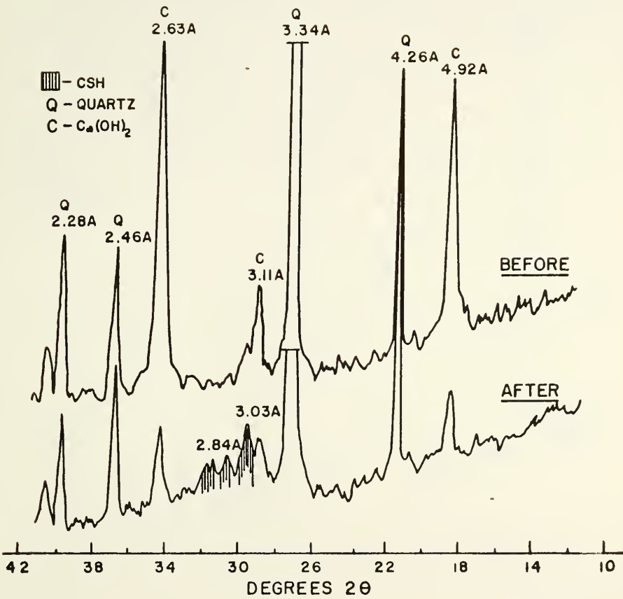
Figure 1-A. X-ray Diffractometer Traces of Quartz- \text{Ca}(\text{OH})_2 Mixture Before and After Reaction at 60^\circ\text{C} .
