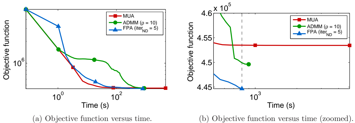
Figure 9: NMF on an excerpt of Armstrong's song.
