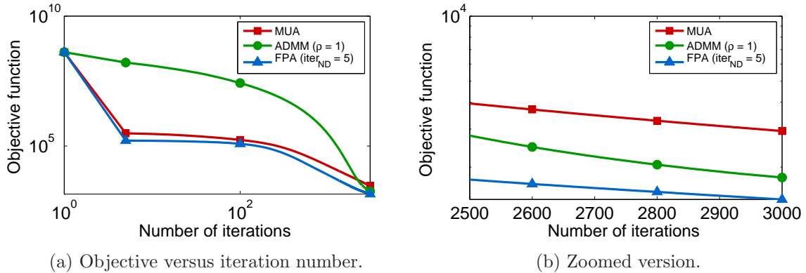
Figure 10: NMF on synthetic data. It is important to recall that the dual function is not presented due to the non-convexity of the NMF problem.
