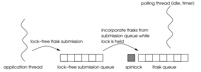
Fig. 1. Submission queues
