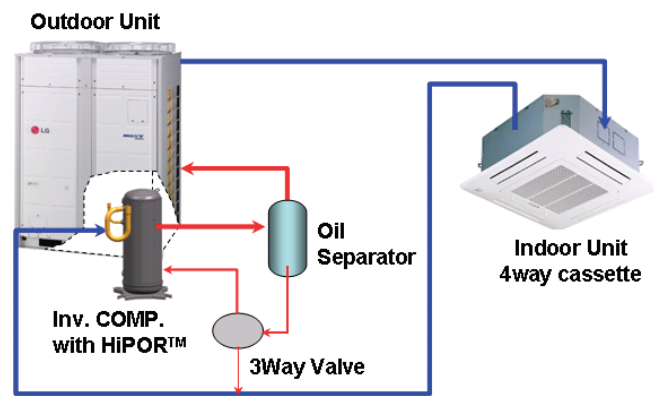
Figure 6 Configuration of Test System
