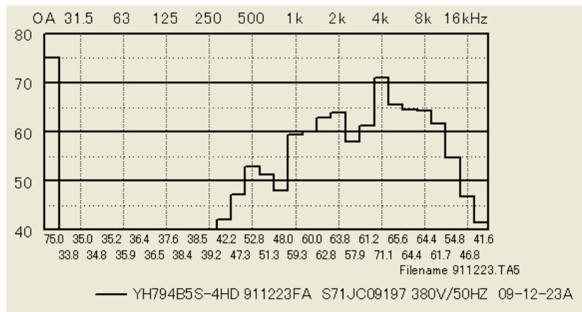
Fig.4 Noise frequency spectrum before optimization
