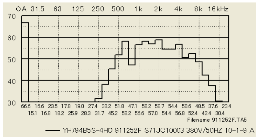
Fig.5 Noise frequency spectrum after optimization
