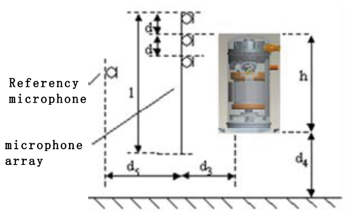
Fig.1 Microphones vertical layout
