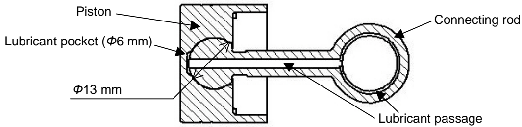
Figure 3: Cross section of ball joint
