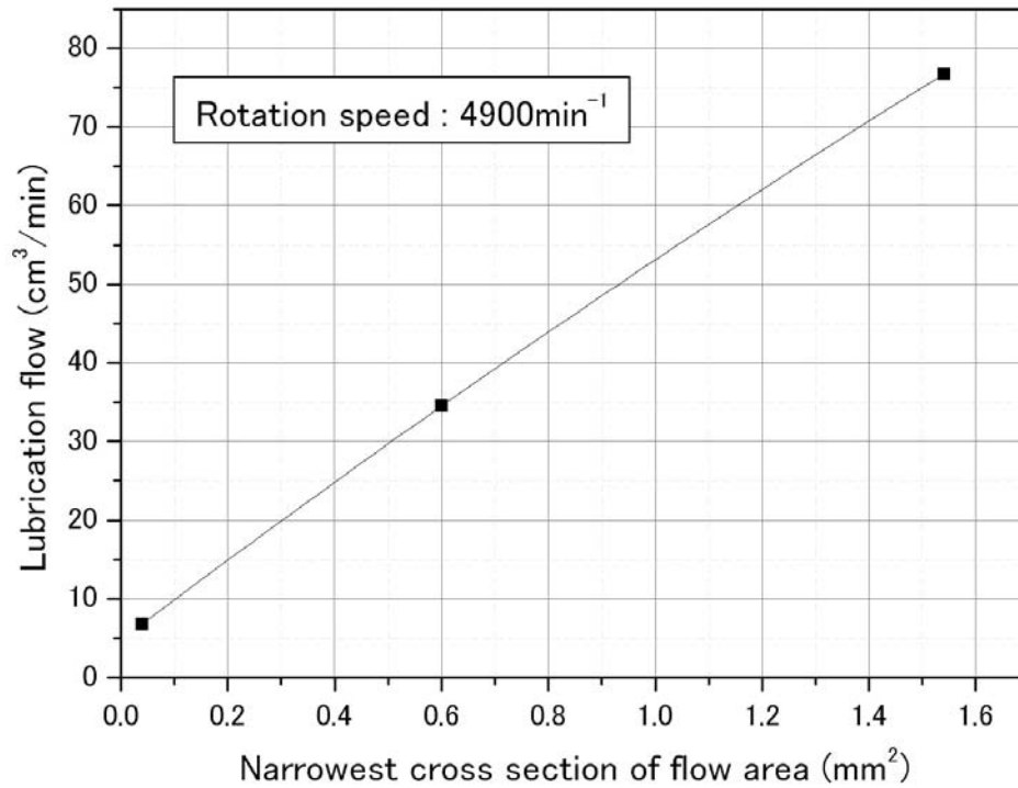
Figure 6: Relationship between lubricant flow and cross section of flow area
