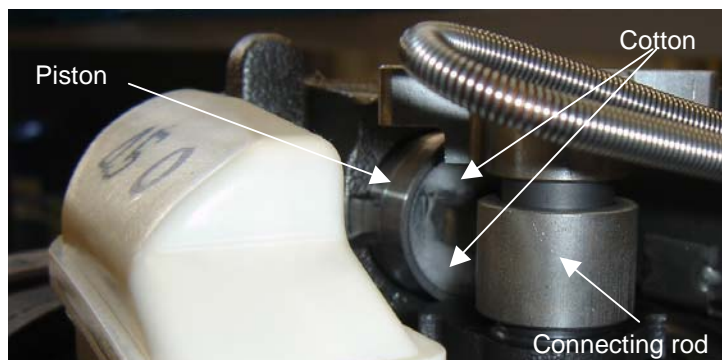
Figure 4: Measuring lubricant flow
