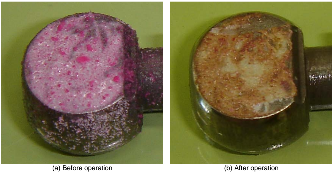
Figure 5: Measuring temperature with THERMO CRAYON
