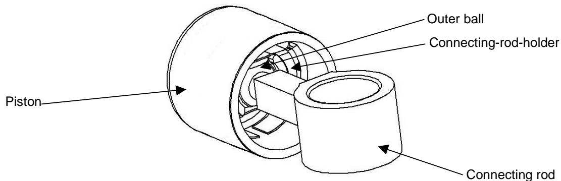
Figure 2: Piston and connecting rod
