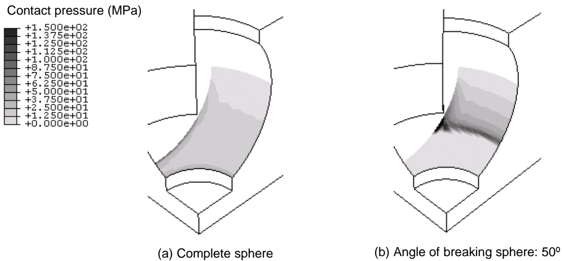
Figure 8: FEA result of piston and connecting rod's outer ball
