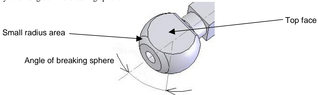
Figure 7: Definition of outer ball's edge angle
