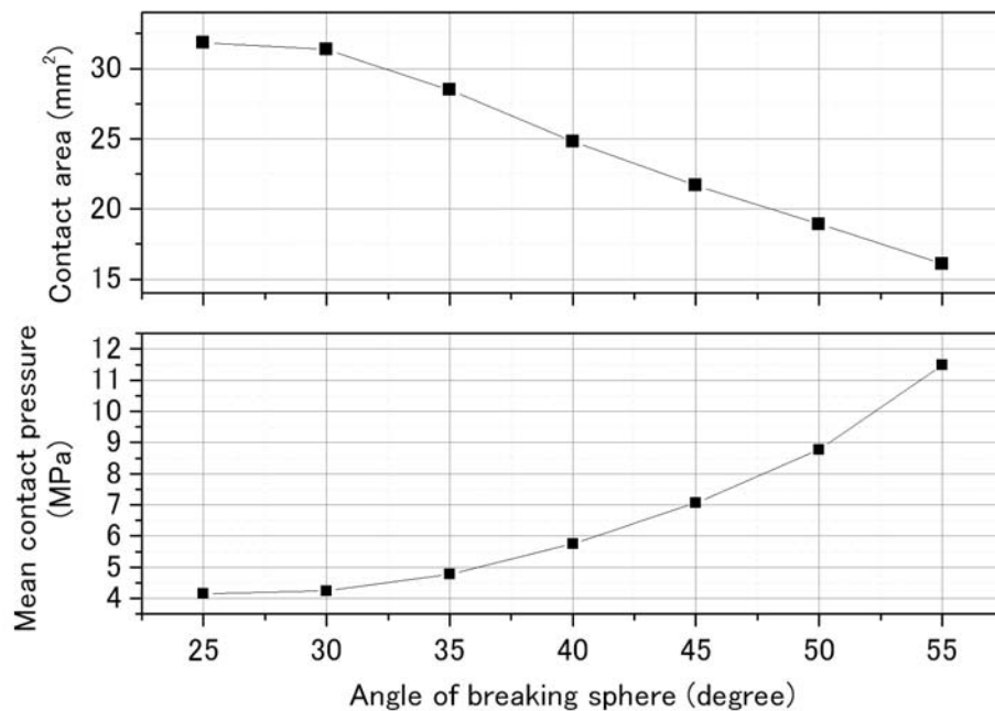
Figure 10: Relationship between contact area, mean contact pressure, and angle of breaking sphere
