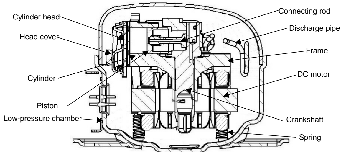
Figure 1: Cross section of reciprocating compressor
