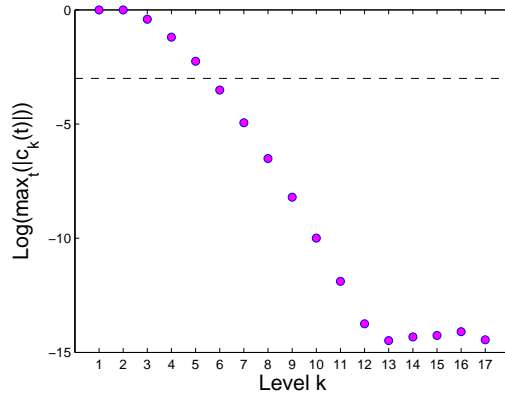
Fig. 2 (Color online) Maxima of populations over the whole dynamics for each level of the planar rotor. The horizontal dashed line indicates the position of the threshold error \varepsilon .
