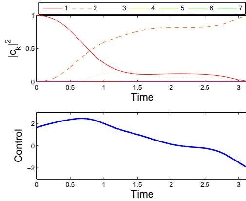
Fig. 1 (Color online) Upper frame: Evolution of the populations during the controlled dynamics. The final distance 1 - |\langle \psi(T) | \psi_f \rangle|^2 to the target state |\psi_f\rangle is 2 \times 10^{-3} . Bottom frame: the corresponding control field, with K = 3.86 .
