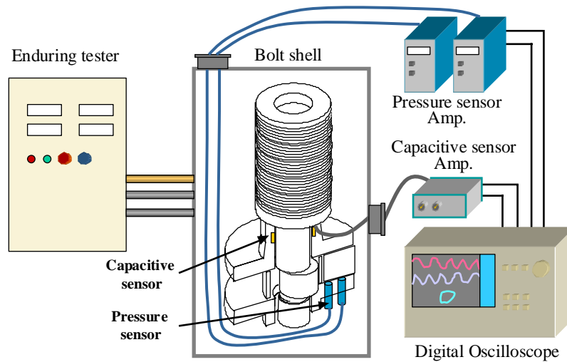
Fig. 6 Schematic of experimental setup
