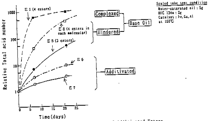
Fig.3 Hydrolysis ability and Structure of Additivated Esters
