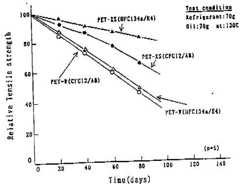
Fig. 6 Change of Tensile strength of Different PET films with Different Refrigerant/Oil systems
