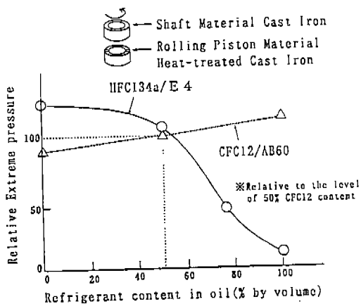
Fig. 7 Influence of Extreme pressure depend on Refrigerant content in Oil
