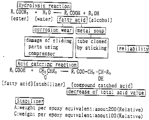
Fig.2 Chemical behavior of Ester for HFC134a refrigerant
