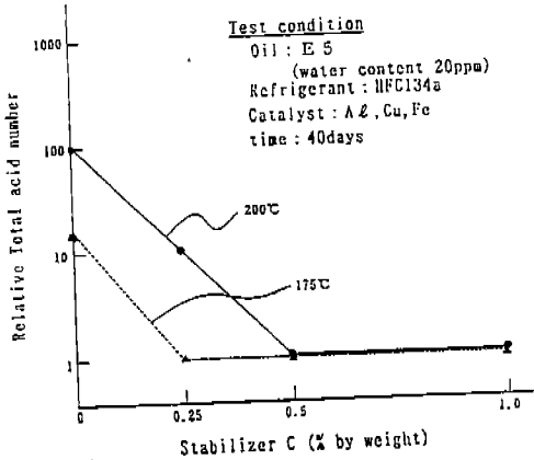
Fig.4 Controlled Total acid number in oil depend on additive
