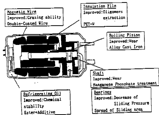
Fig. 8 Structure of new rotary type compressor for HFC134a
