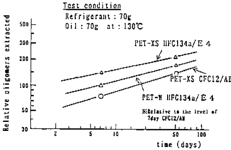
Fig. 5 Level of oligomers Extracted from Different PET Film with Different Refrigerant/Oil systems
