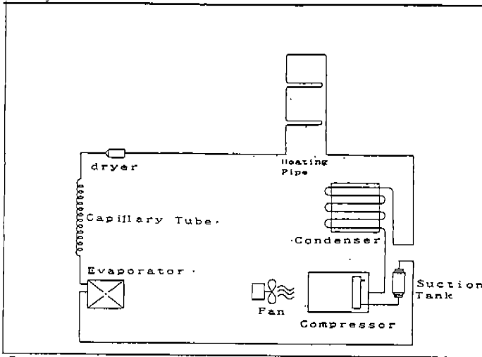
Fig. 9 Refrigeration piping system for domestic refrigeration
