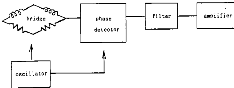
Fig. 3 Circuit diagram
