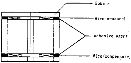
Fig. 1 Sensor structure
