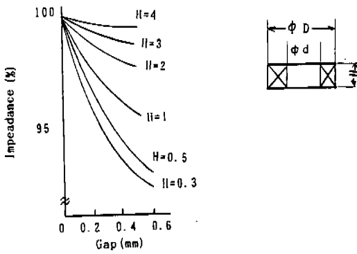
Fig. 2 Characteristic of gap sensor
