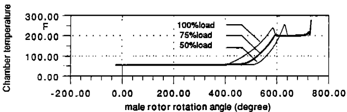
Figure 7: Chamber Temperature
