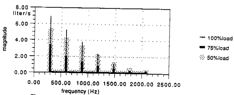
Figure 12: Fourier Components of the Discharge Flow Pulsation
