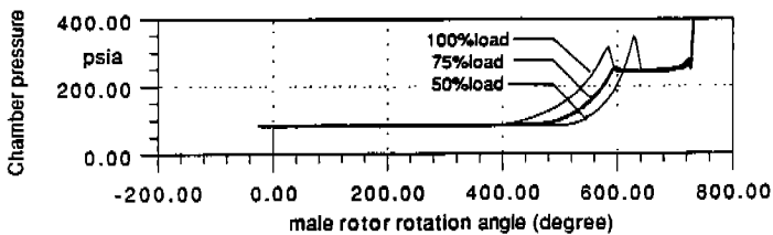
Figure 6: Chamber Pressure
