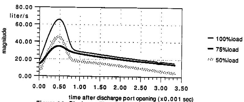
Figure 11: Discharge Flow Pulsation in One Period
