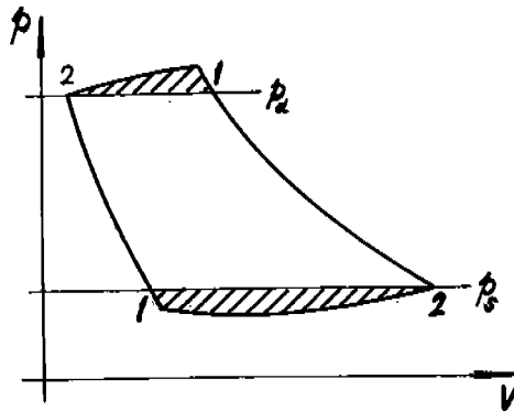
Fig. 1. Pressure-volume diagram calculating idealized valve loss work
